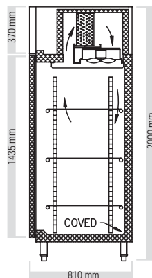
CROSS SECTION
