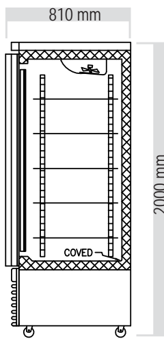
CROSS SECTION
