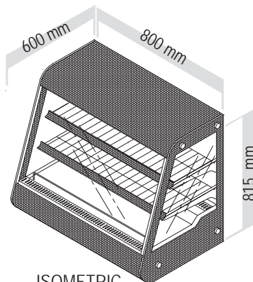
ISOMETRIC
