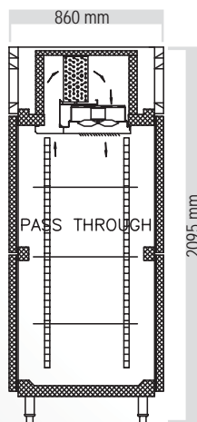
CROSS SECTION
