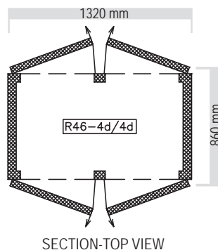
SECTION-TOP VIEW
